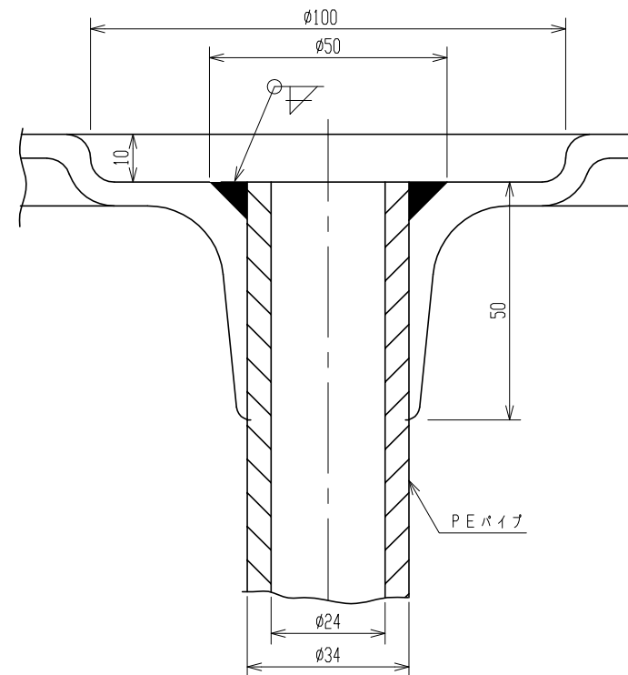
D 部詳細 (S = 1 / 1)
