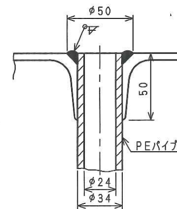
△ B部詳細 (S=1/2)
