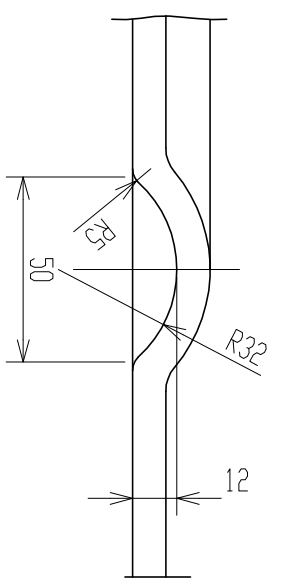
B部詳細 (S = 1 / 2)
